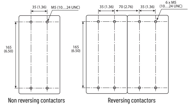
Figure 84 - 100-E265...100-E370 Contactors
