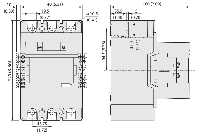
Figure 84 - 100-E265...100-E370 Contactors
