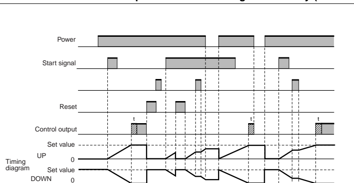
Output mode A Mode: Signal ON-Delay (Timer resets when power comes ON.)
