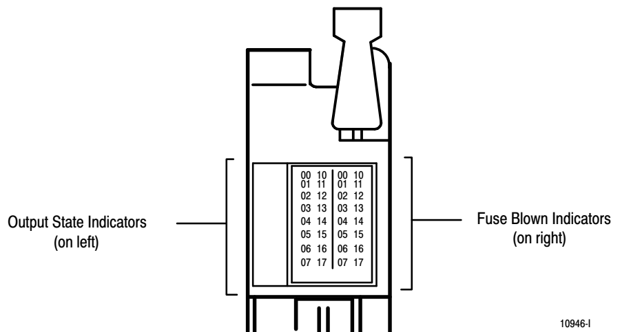
Figure 3 Status Indicators
