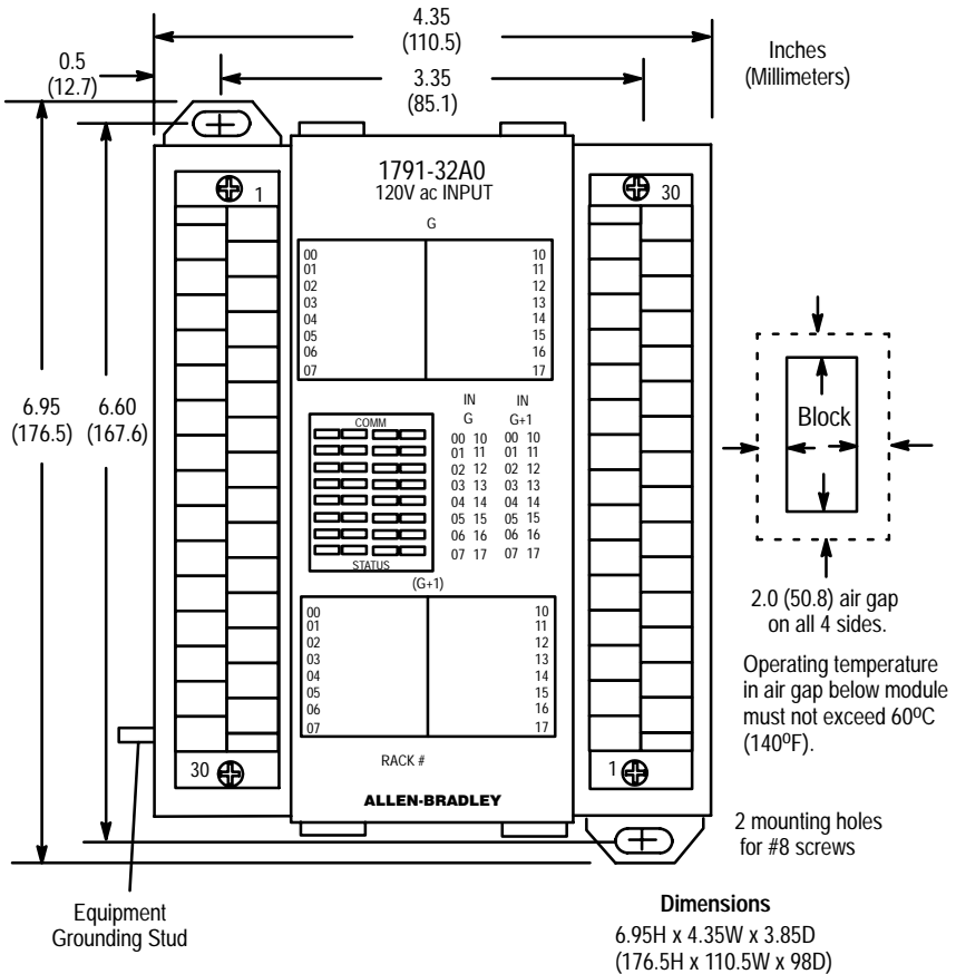
Figure 1 Mounting Dimensions for the Block I/O Module Cat. No. 1791-32A0 (PLC version shown)
